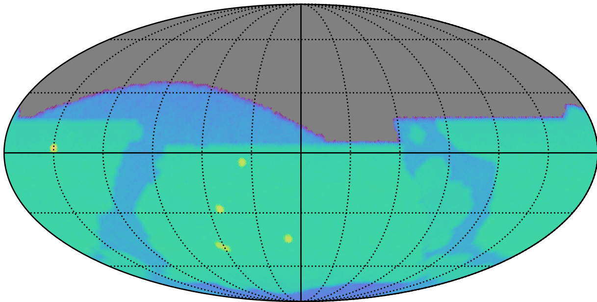
weather_cloudso1v3.4_10yrs z: SurfaceBrightLimit
