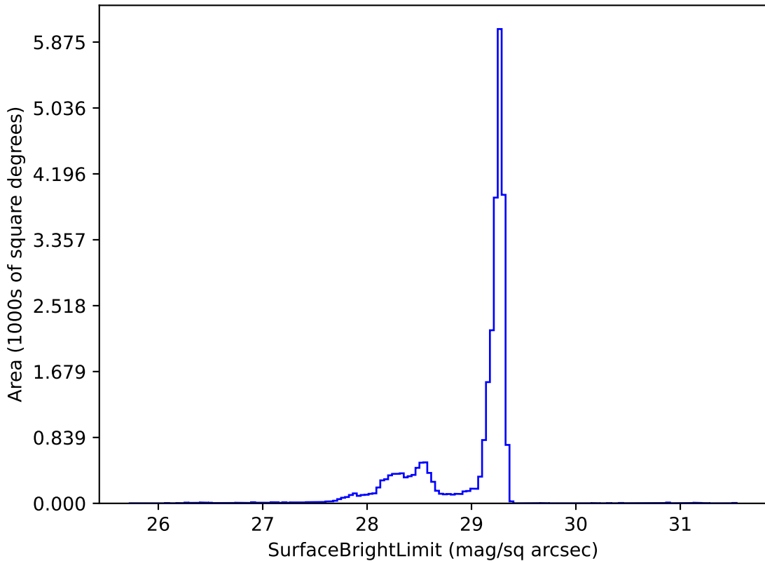
weather_cloudso1v3.4_10yrs z: SurfaceBrightLimit
