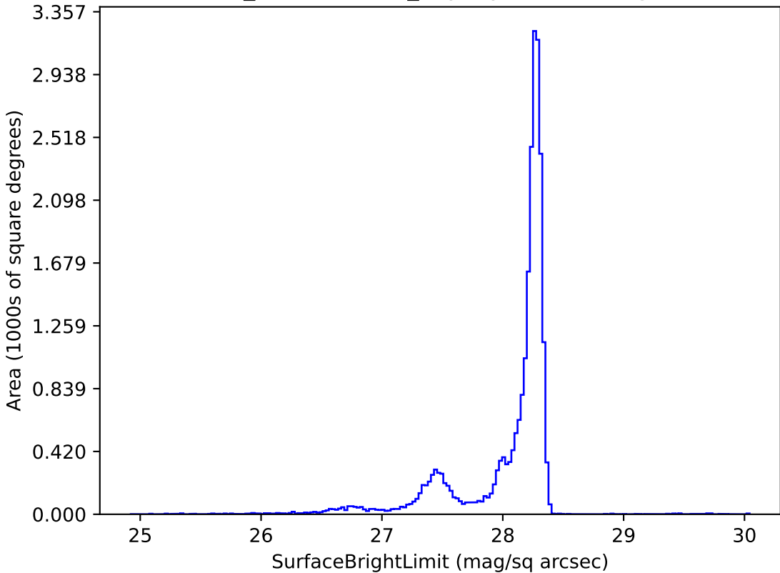
weather_cloudso1v3.4_10yrs y: SurfaceBrightLimit
