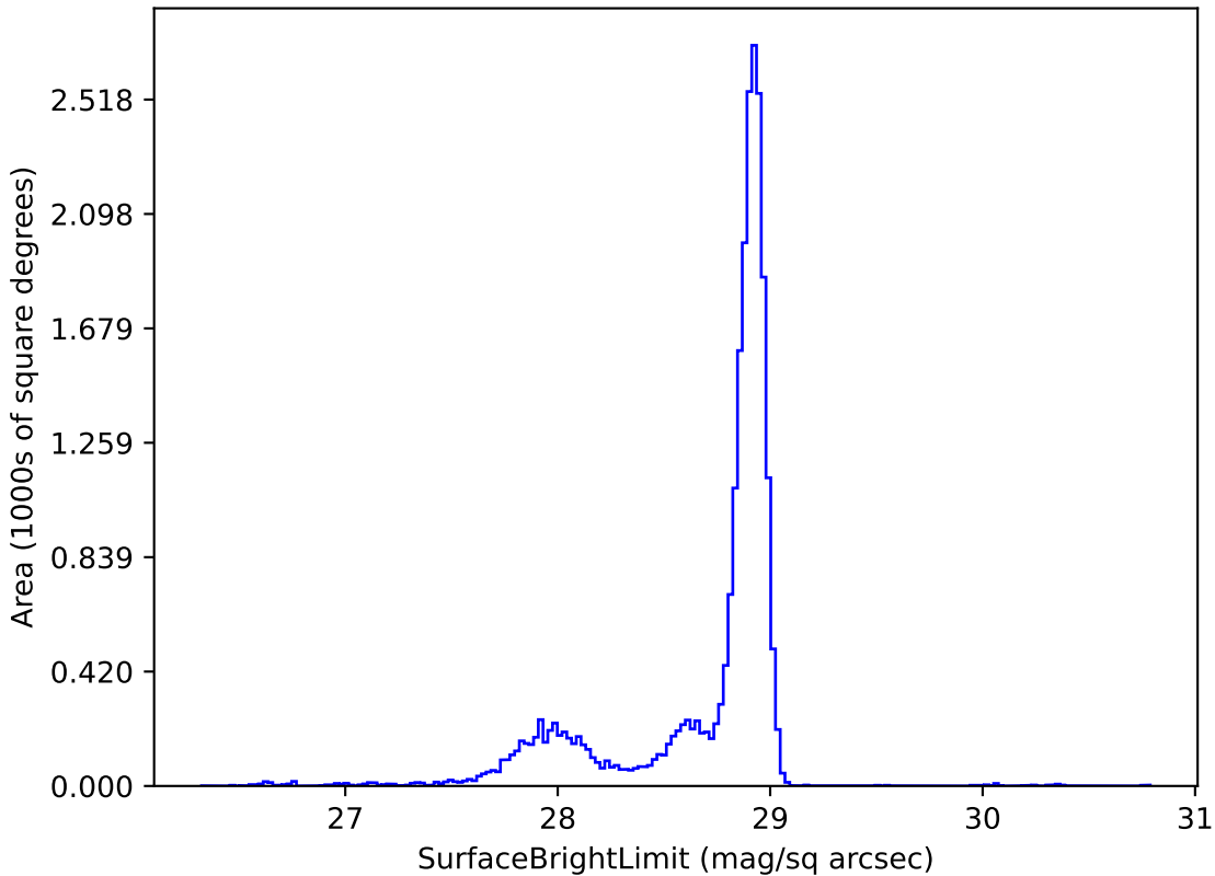
weather_cloudso1v3.4_10yrs u: SurfaceBrightLimit
