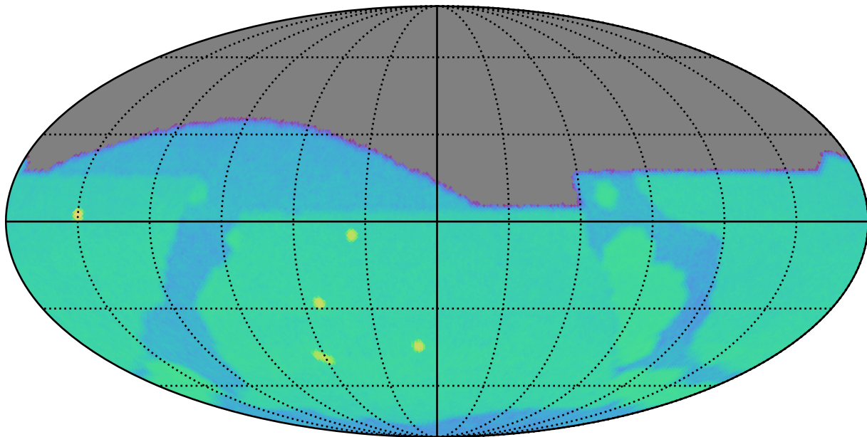
weather_cloudso1v3.4_10yrs g: SurfaceBrightLimit
