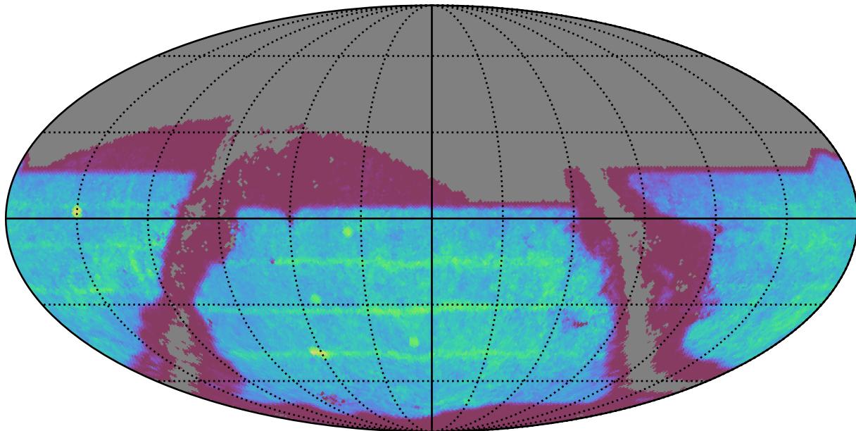
weather_cloudso1v3.4_10yrs : SNSLMetric
