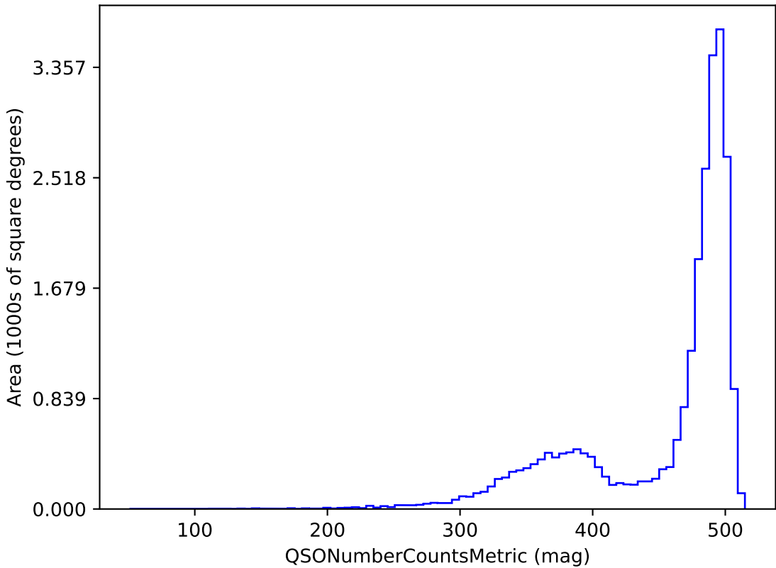
weather_cloudso1v3.4_10yrs z band and non-DD: QSONumberCountsMetric
