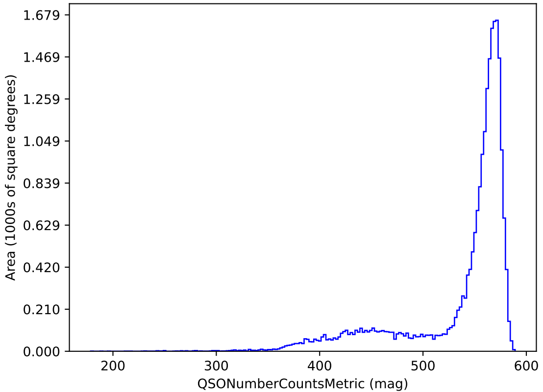
weather_cloudso1v3.4_10yrs y band and non-DD: QSONumberCountsMetric
