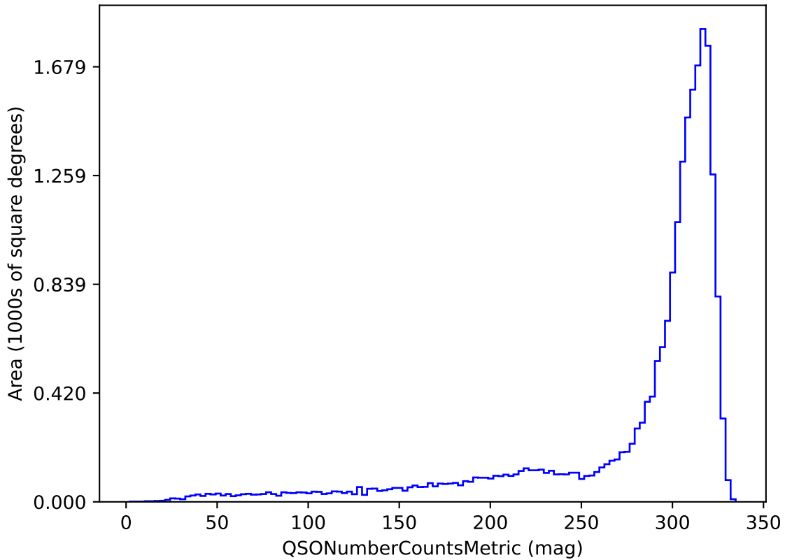
weather_cloudso1v3.4_10yrs u band and non-DD: QSONumberCountsMetric
