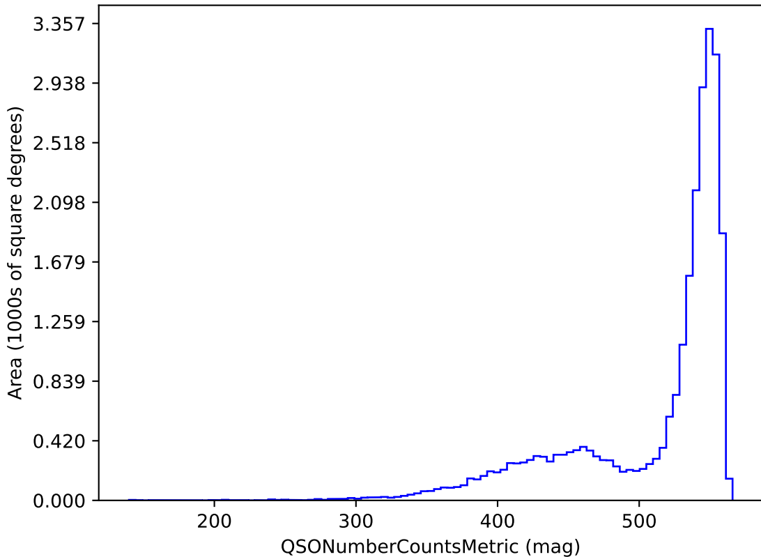
weather_cloudso1v3.4_10yrs i band and non-DD: QSONumberCountsMetric
