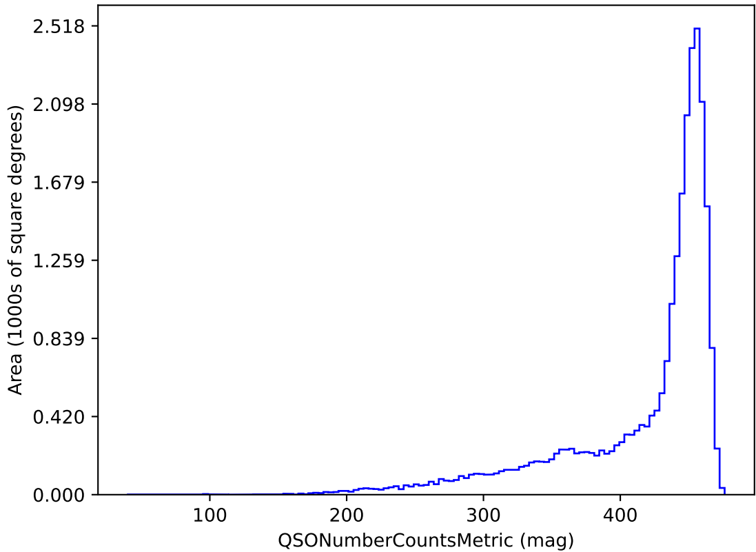
weather_cloudso1v3.4_10yrs g band and non-DD: QSONumberCountsMetric
