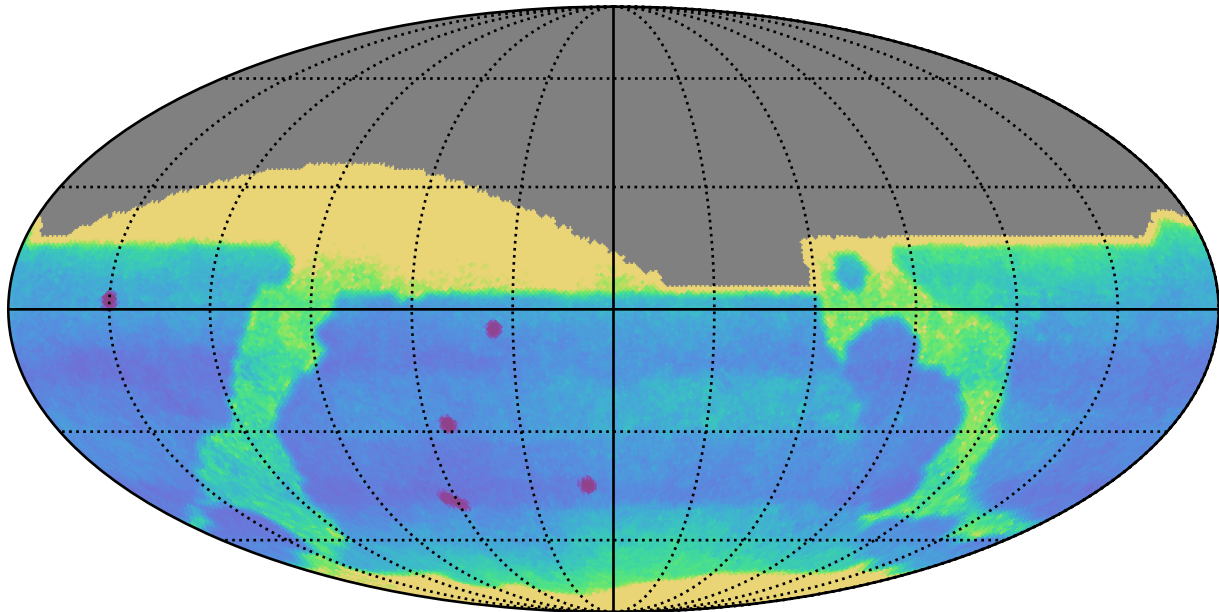
weather_cloudso1v3.4_10yrs : Proper Motion Uncert @ 24.0
