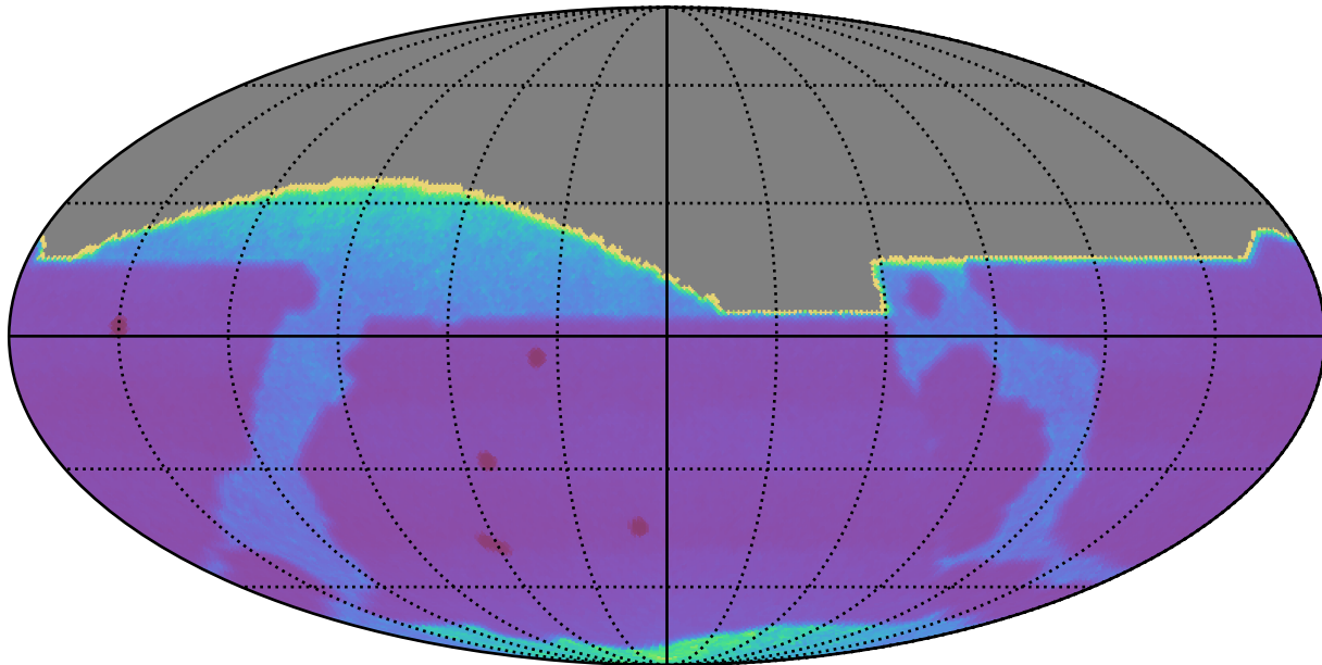
weather_cloudso1v3.4_10yrs : Proper Motion Uncert @ 20.5
