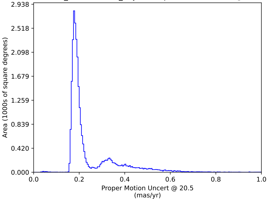
weather_cloudso1v3.4_10yrs : Proper Motion Uncert @ 20.5
