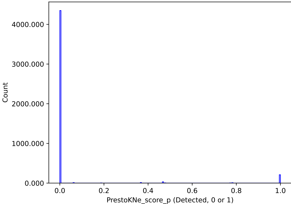
weather_cloudso1v3.4_10yrs : PrestoKNe_score_p
