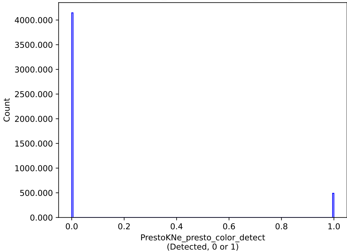
weather_cloudso1v3.4_10yrs : PrestoKNe_presto_color_detect
