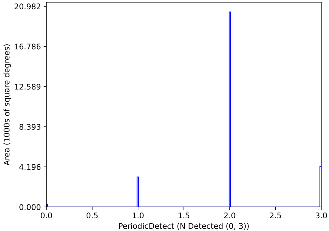
weather_cloudso1v3.4_10yrs P_1.0_Mag_21_Amp_0.05-0.1-1 Yr 2: PeriodicDetect
