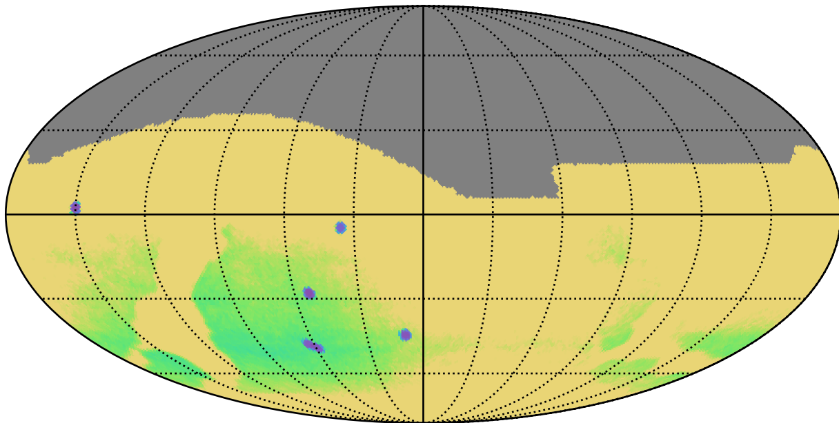
weather_cloudso1v3.4_10yrs : Parallax Uncert @ 22.4
