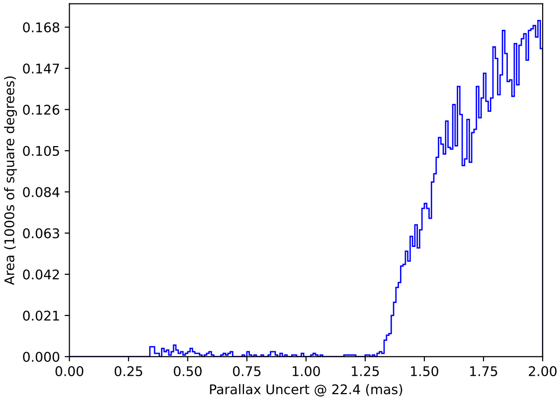
weather_cloudso1v3.4_10yrs : Parallax Uncert @ 22.4
