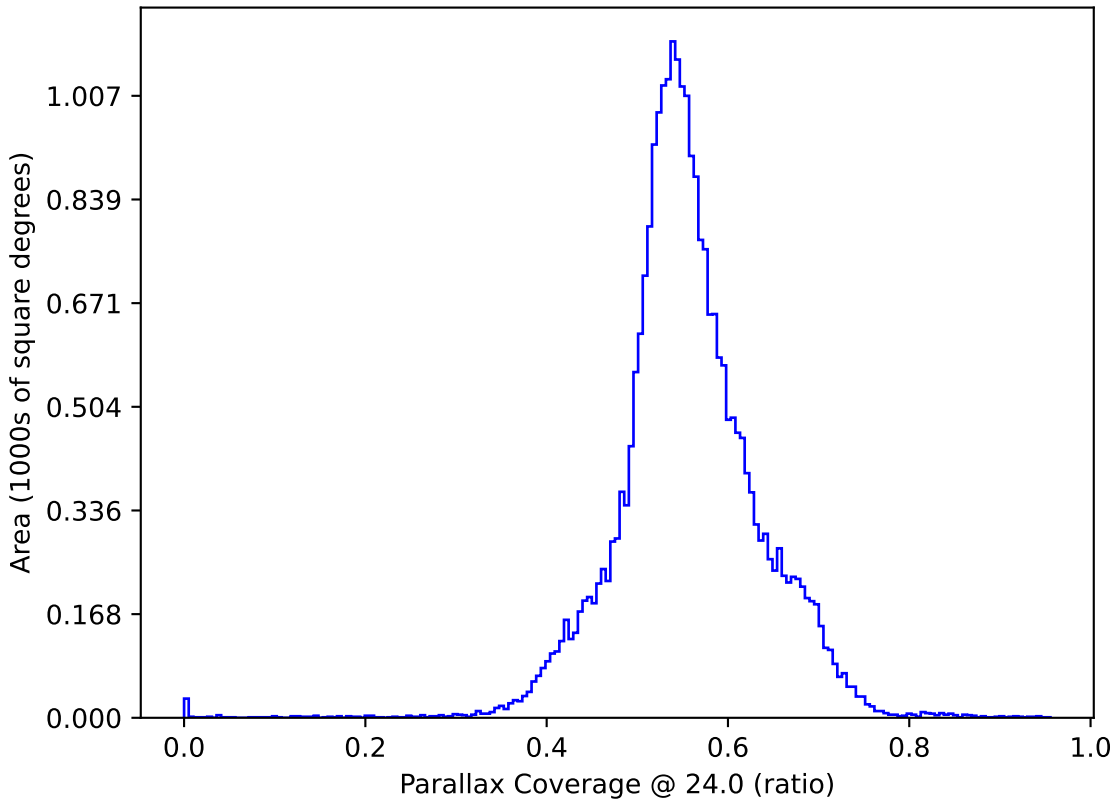
weather_cloudso1v3.4_10yrs : Parallax Coverage @ 24.0
