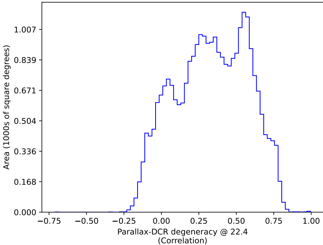
weather_cloudso1v3.4_10yrs : Parallax-DCR degeneracy @ 22.4
