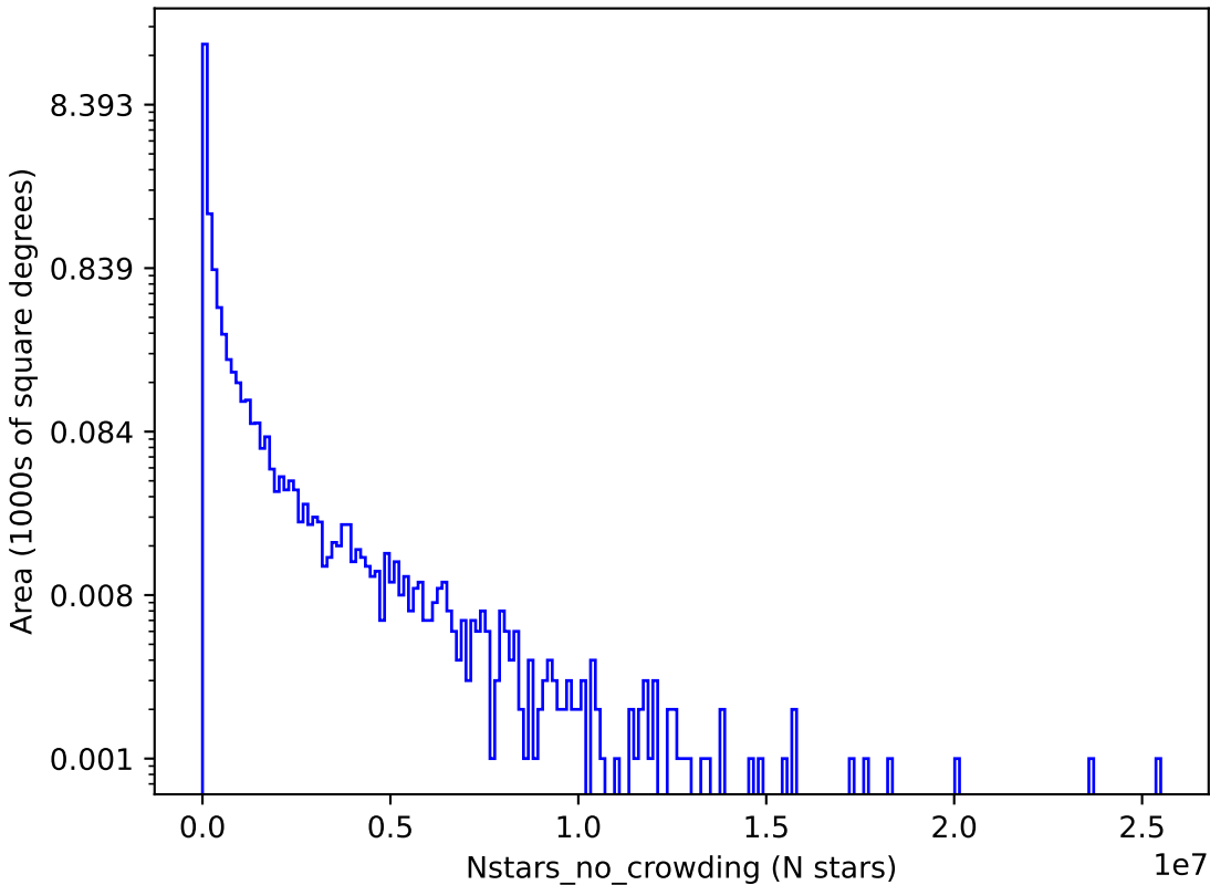
weather_cloudso1v3.4_10yrs y: Nstars_no_crowding
