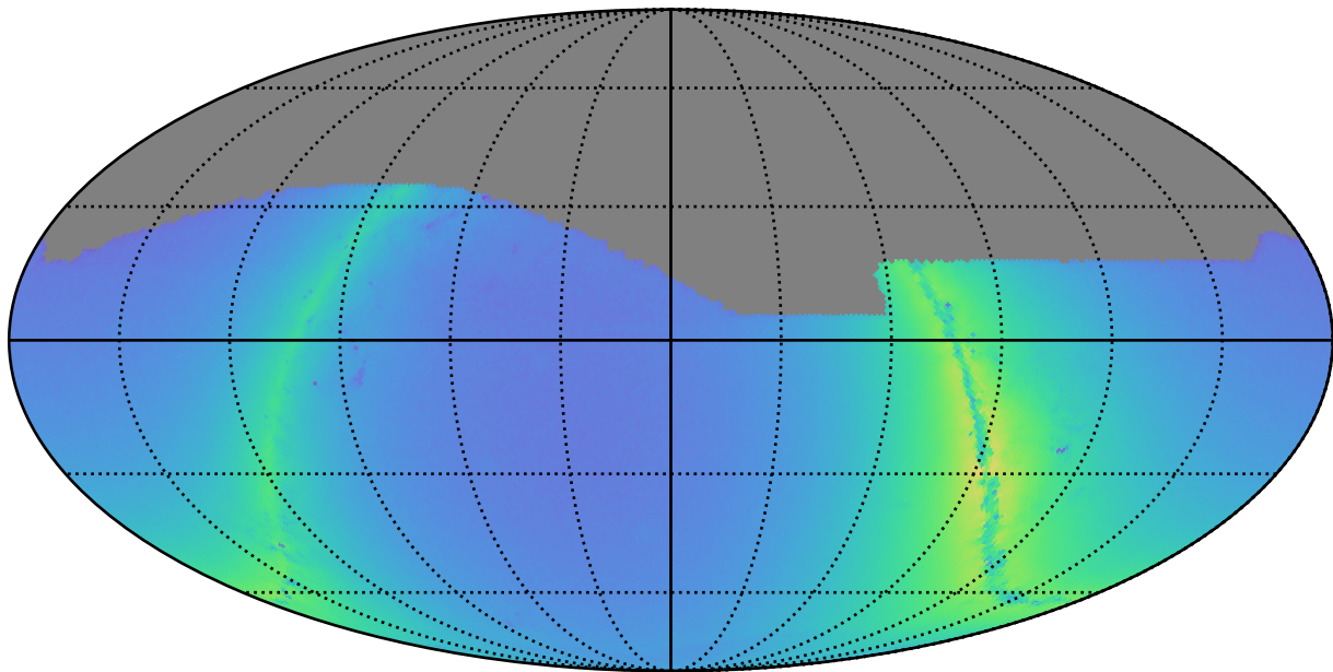
weather_cloudso1v3.4_10yrs r: Nstars_no_crowding
