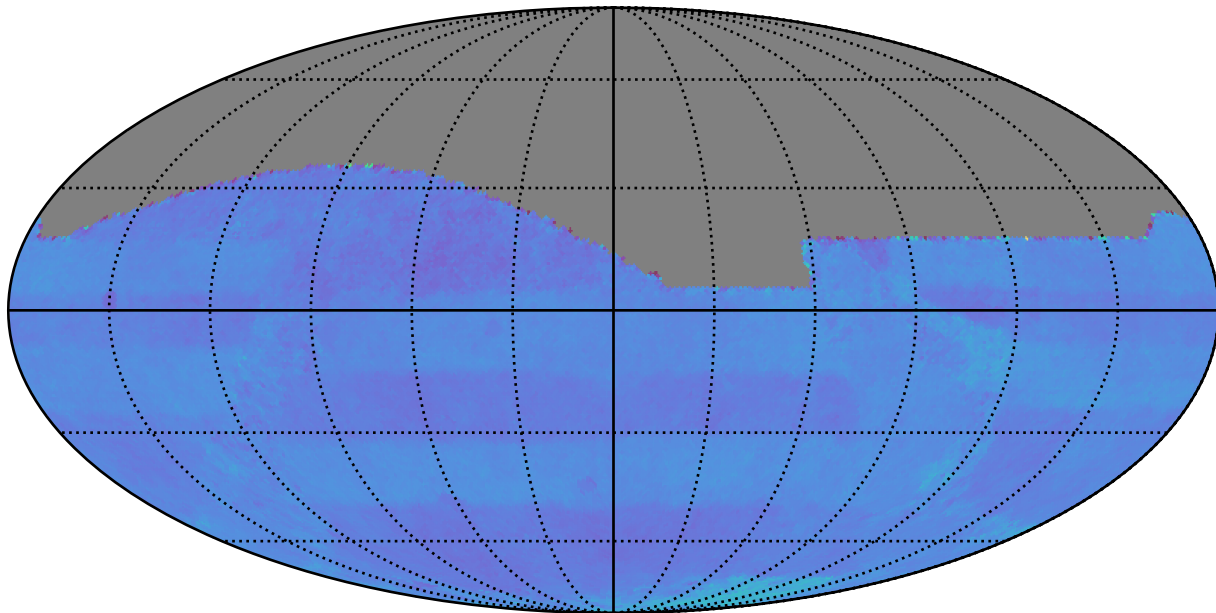
weather_cloudso1v3.4_10yrs : Normalized Proper Motion Uncert @ 24.0
