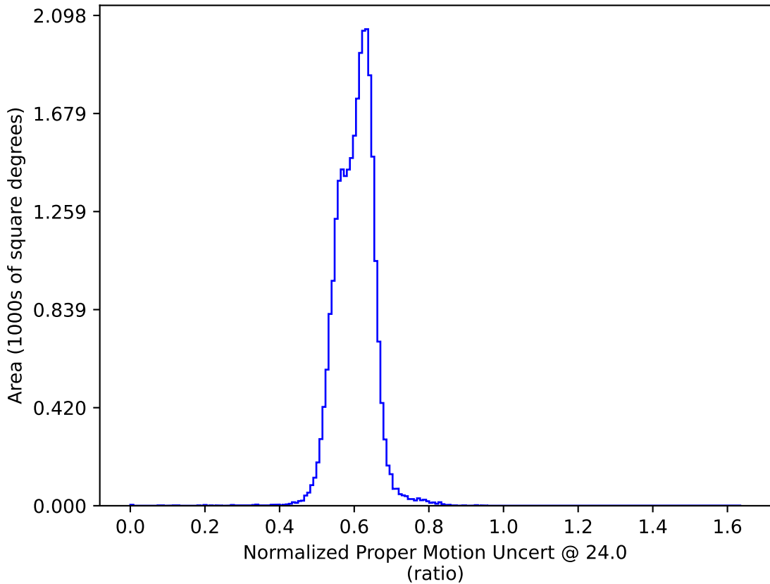
weather_cloudso1v3.4_10yrs : Normalized Proper Motion Uncert @ 24.0
