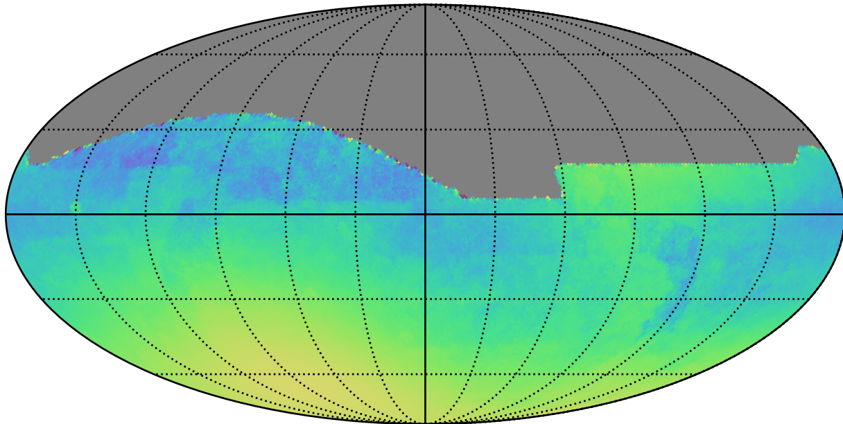
weather_cloudso1v3.4_10yrs : Normalized Parallax Uncert @ 24.0
