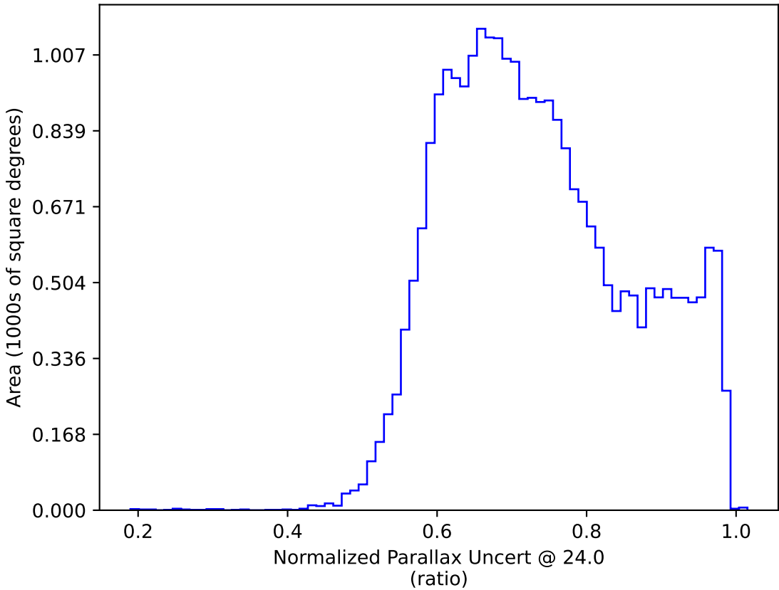
weather_cloudso1v3.4_10yrs : Normalized Parallax Uncert @ 24.0
