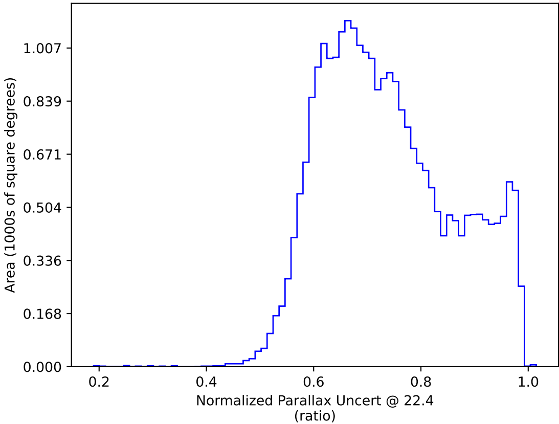
weather_cloudso1v3.4_10yrs : Normalized Parallax Uncert @ 22.4
