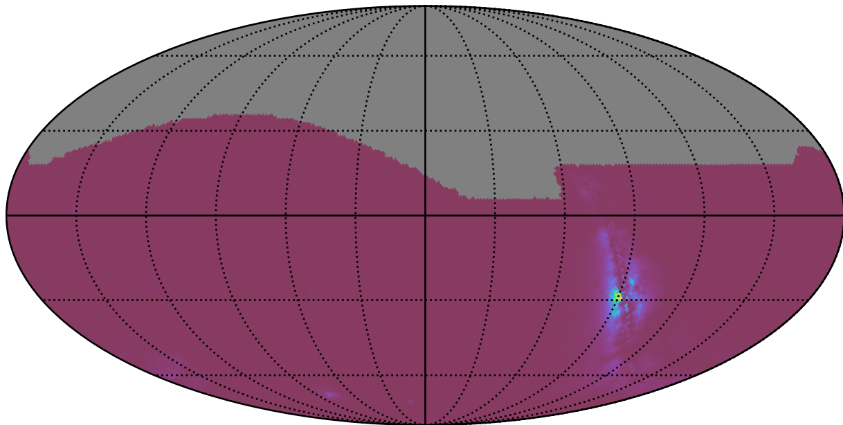
weather_cloudso1v3.4_10yrs : NlcPoints
