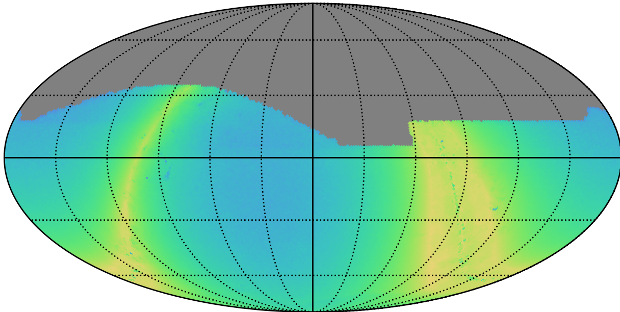
weather_cloudso1v3.4_10yrs z: N stars to Precision 0.20
