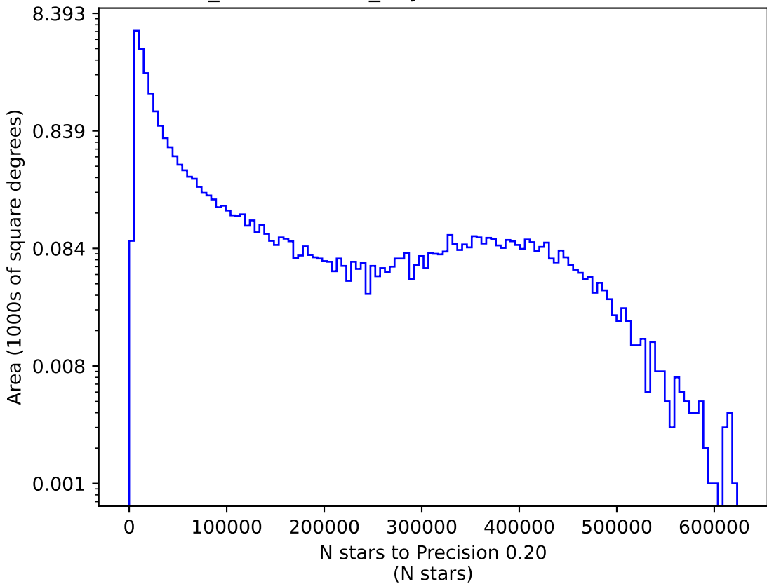
weather_cloudso1v3.4_10yrs z: N stars to Precision 0.20
