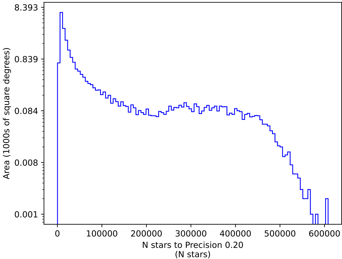
weather_cloudso1v3.4_10yrs y: N stars to Precision 0.20
