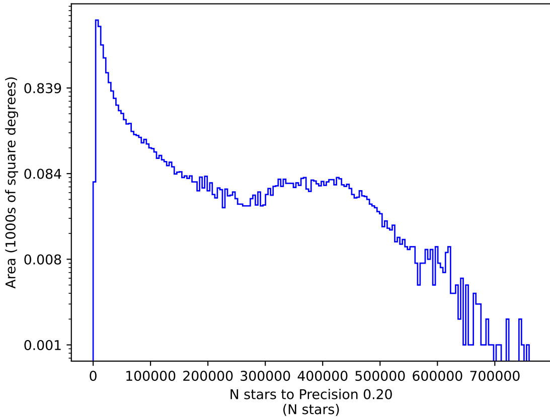
weather_cloudso1v3.4_10yrs r: N stars to Precision 0.20
