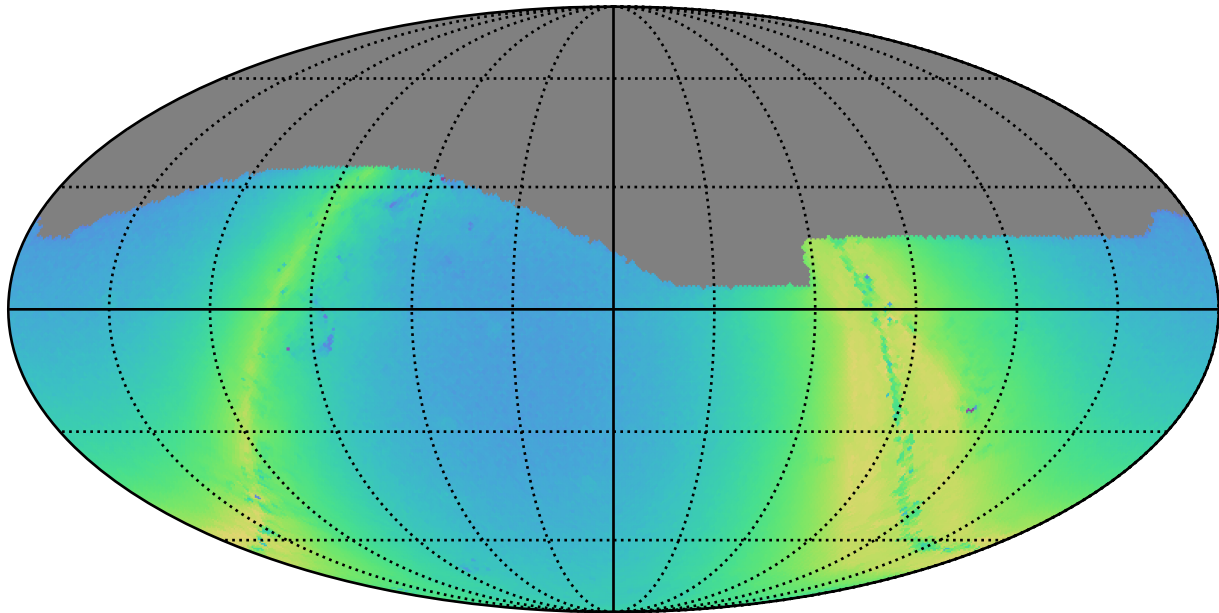
weather_cloudso1v3.4_10yrs g: N stars to Precision 0.20
