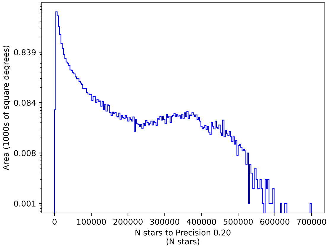
weather_cloudso1v3.4_10yrs g: N stars to Precision 0.20
