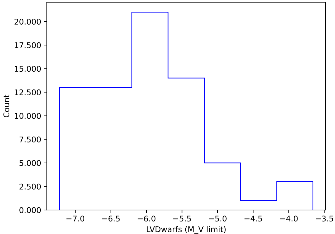
weather_cloudso1v3.4_10yrs gi: LVDwarfs
