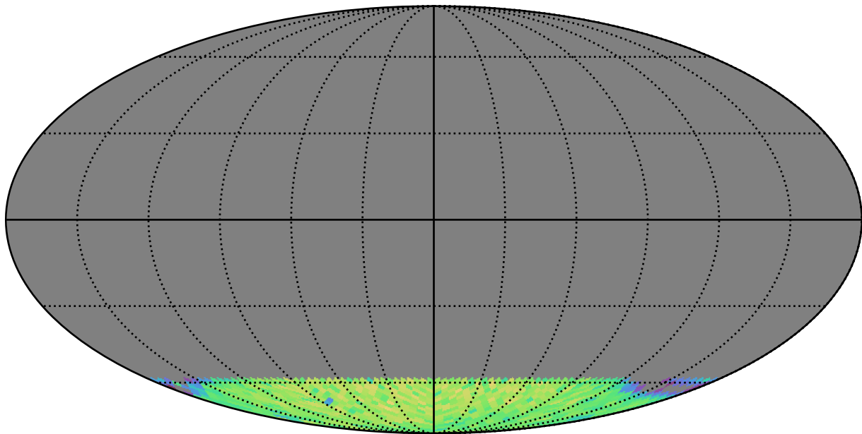
weather_cloudso1v3.4_10yrs gi SCP: LVDwarfs
