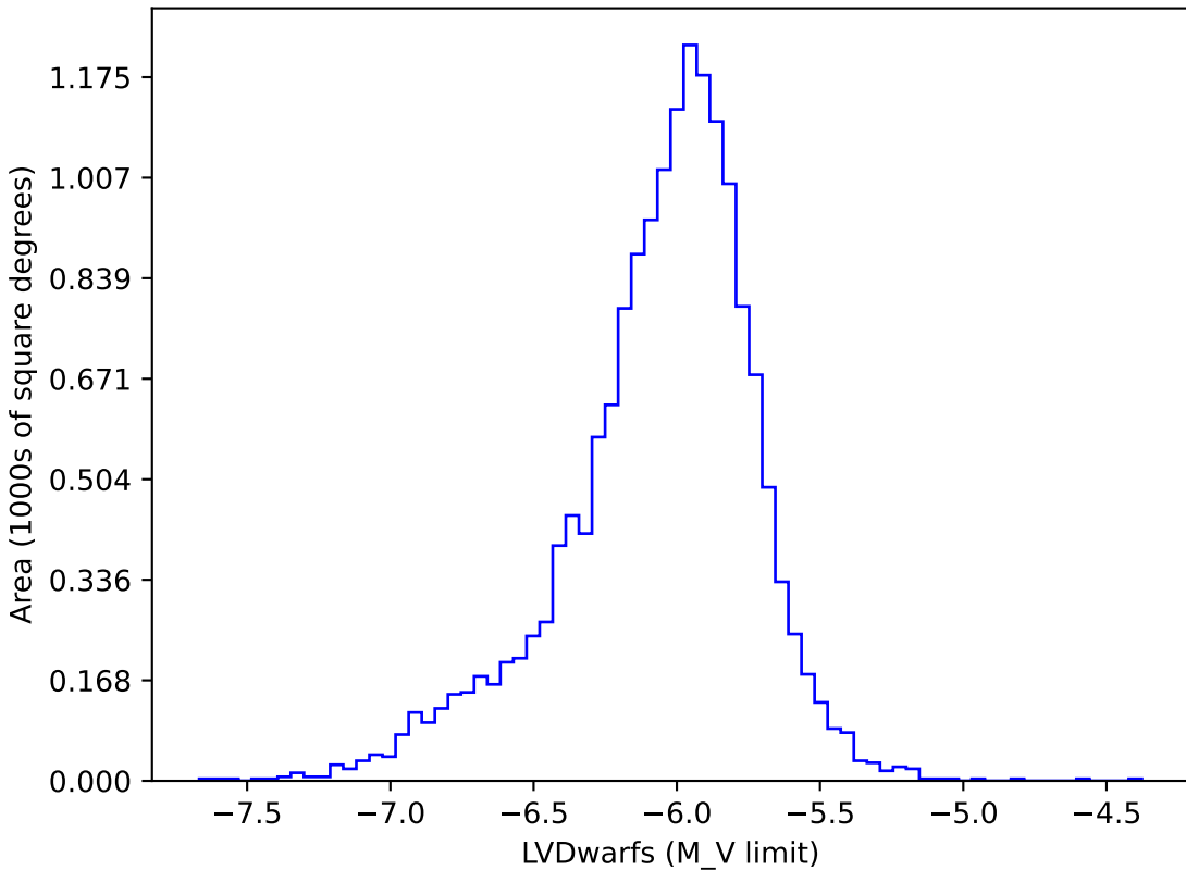
weather_cloudso1v3.4_10yrs gi: LVDwarfs
