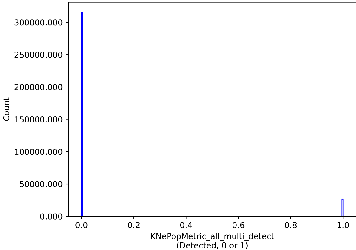
weather_cloudso1v3.4_10yrs all models: KNePopMetric_all_multi_detect
