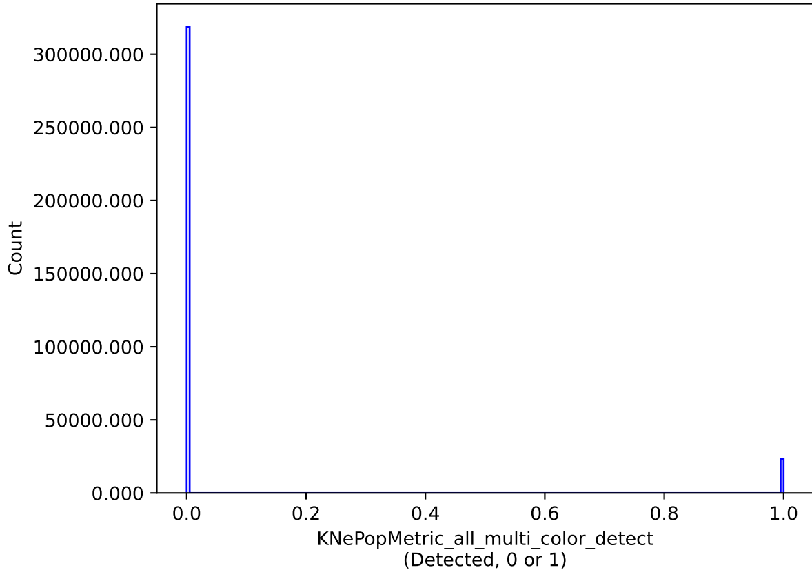
weather_cloudso1v3.4_10yrs all models: KNePopMetric_all_multi_color_detect
