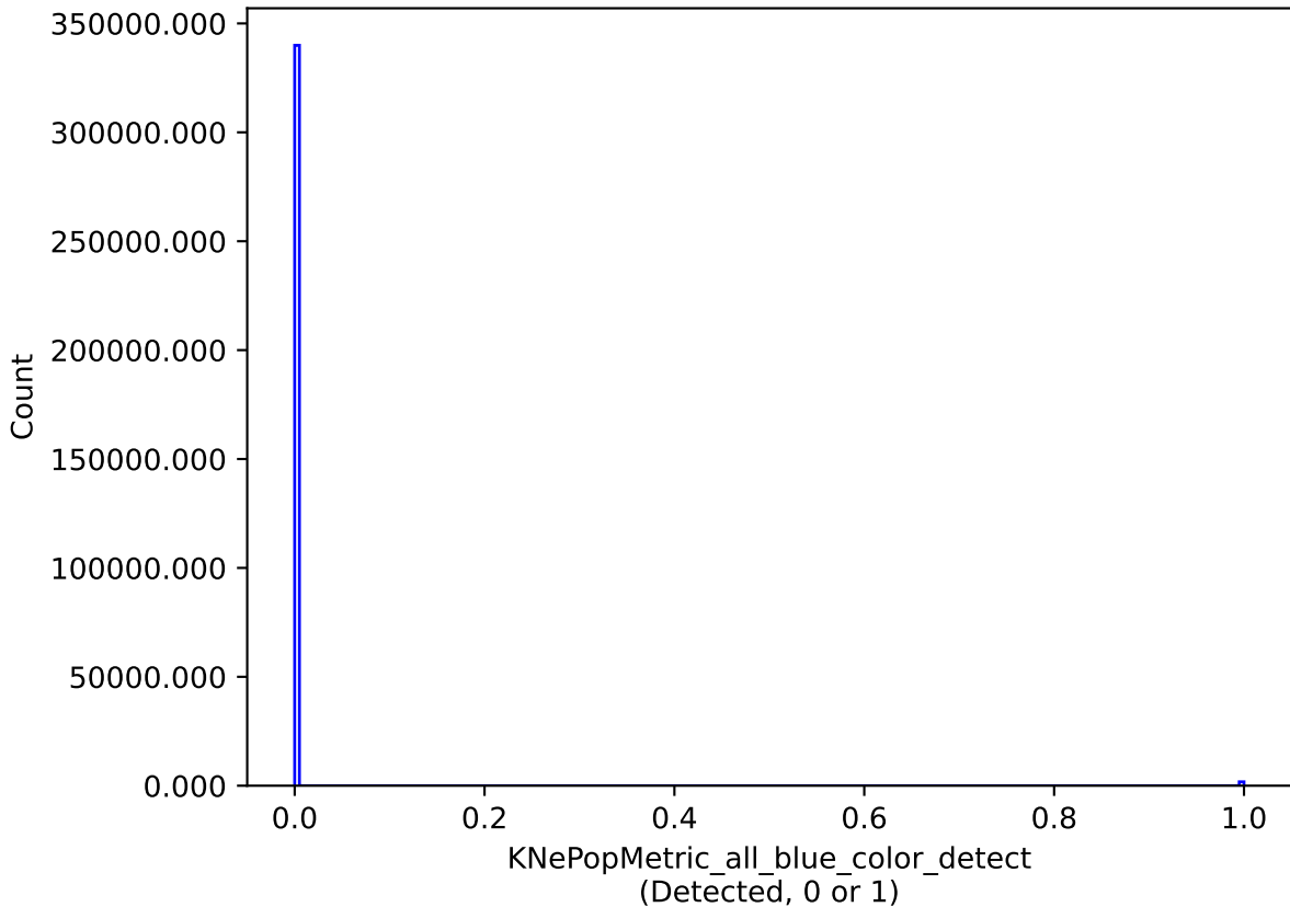
weather_cloudso1v3.4_10yrs all models: KNePopMetric_all_blue_color_detect
