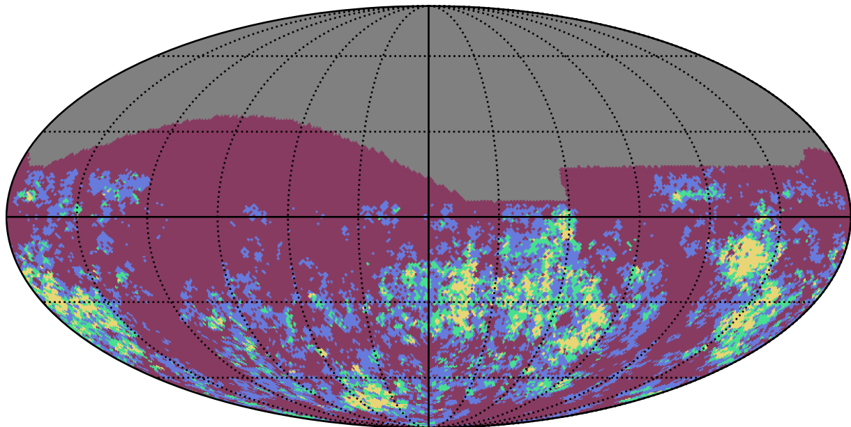
weather_cloudso1v3.4_10yrs z band: Gaps_7hr
