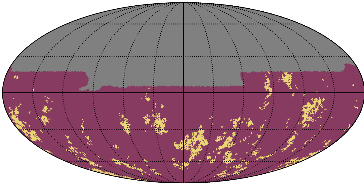
weather_cloudso1v3.4_10yrs u band: Gaps_7hr
