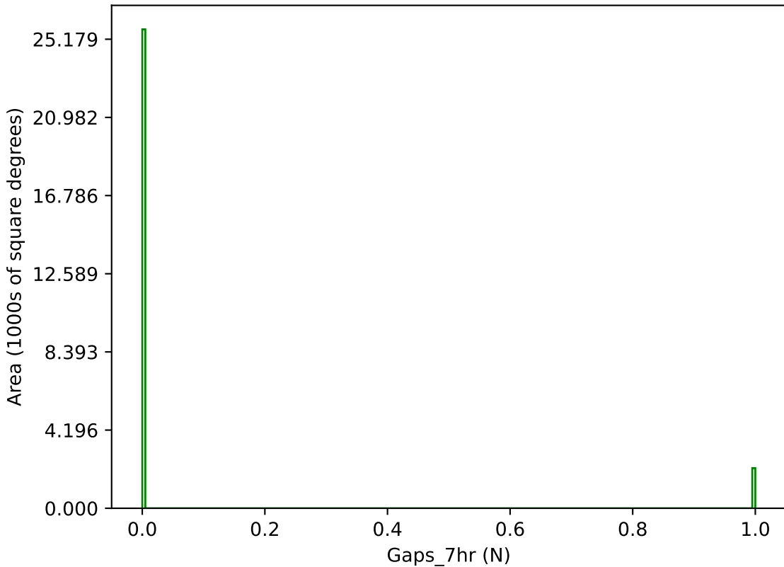
weather_cloudso1v3.4_10yrs g band: Gaps_7hr
