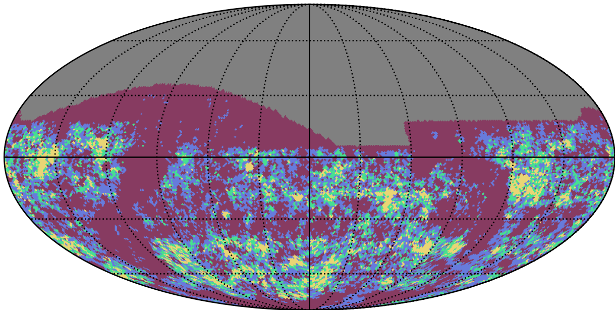
weather_cloudso1v3.4_10yrs z band: Gaps_3hr
