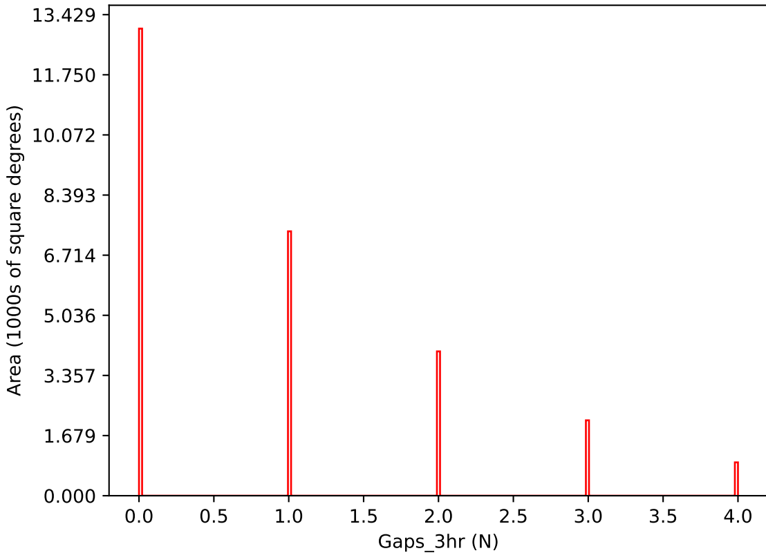
weather_cloudso1v3.4_10yrs i band: Gaps_3hr
