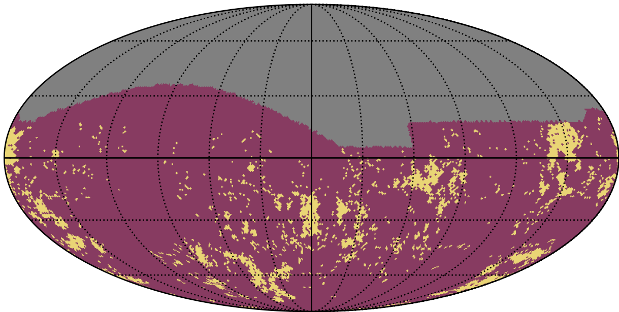
weather_cloudso1v3.4_10yrs g band: Gaps_3hr
