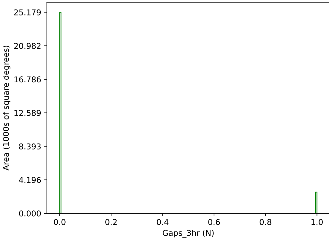
weather_cloudso1v3.4_10yrs g band: Gaps_3hr
