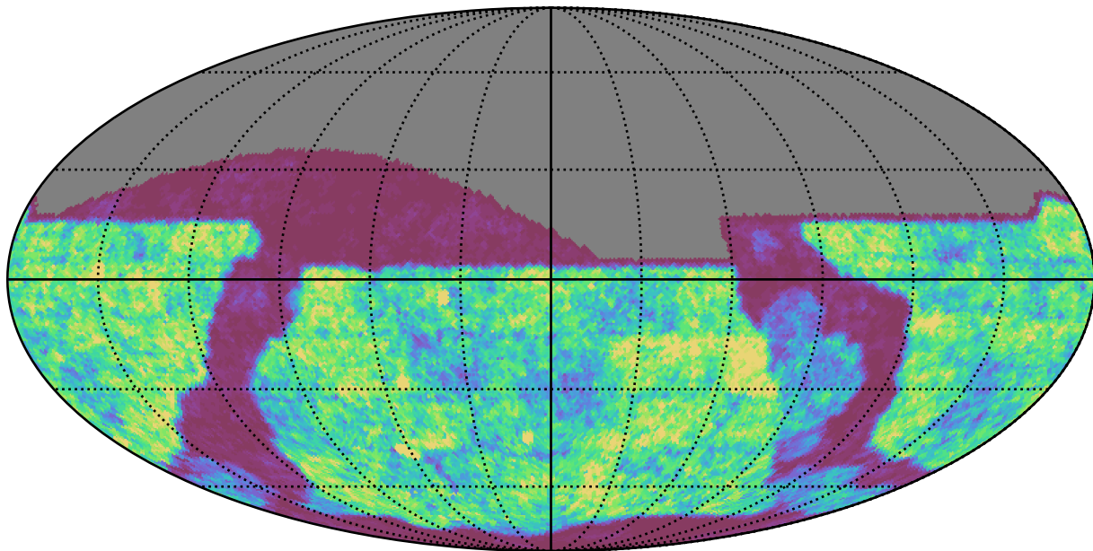
weather_cloudso1v3.4_10yrs z band: Gaps_24hr
