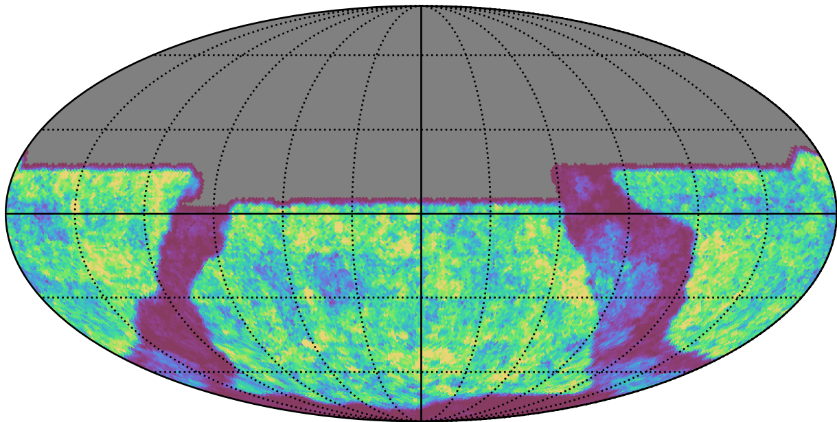
weather_cloudso1v3.4_10yrs y band: Gaps_24hr
